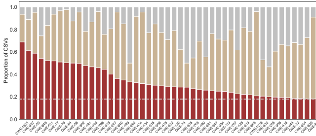
Figure 5: CSV proportion of each CWE category. The red, yellow, and gray bar represents the CRITICAL, HIGH, and MEDIUM SVs, respectively. The gray dotted line represents the average proportion of CSV in the entire dataset.
