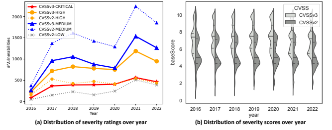
Figure 4: Distribution of severity ratings and scores over years
